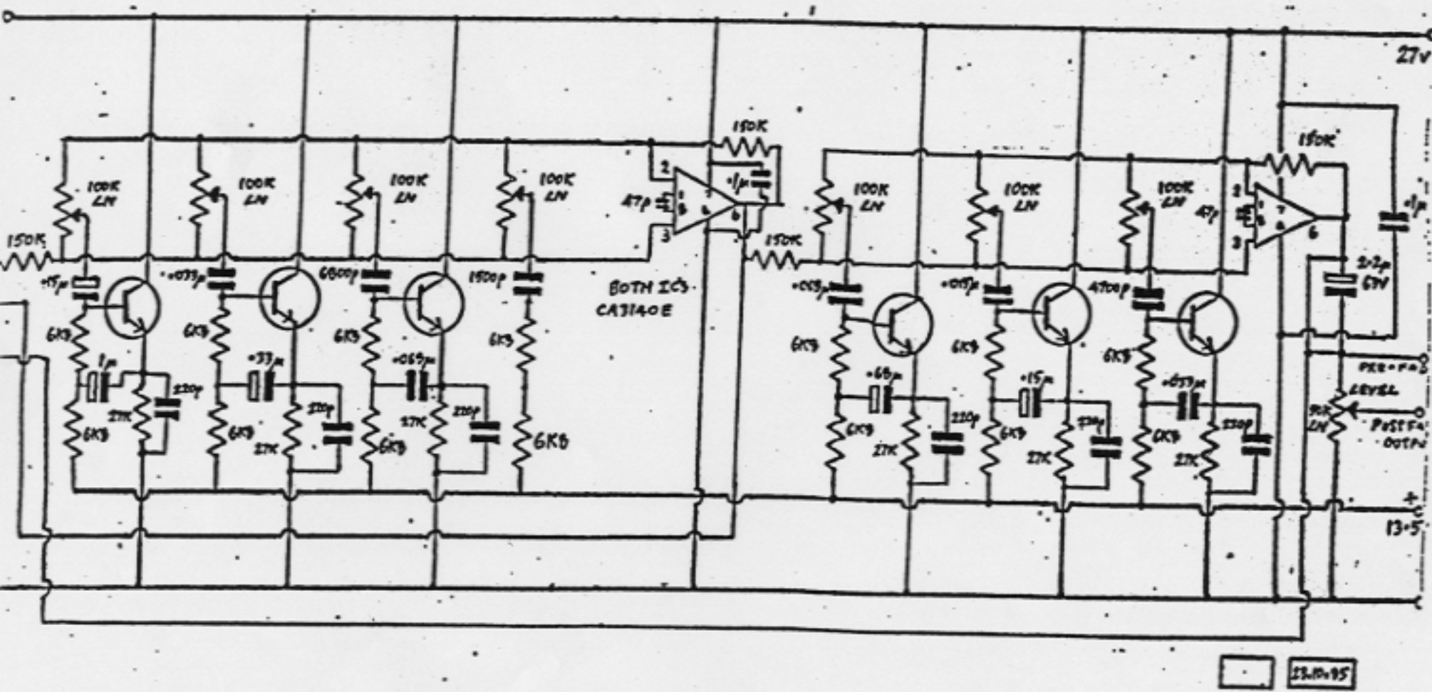
① TRACE ELLIOT GP7 GRAPHIC STAGE.
