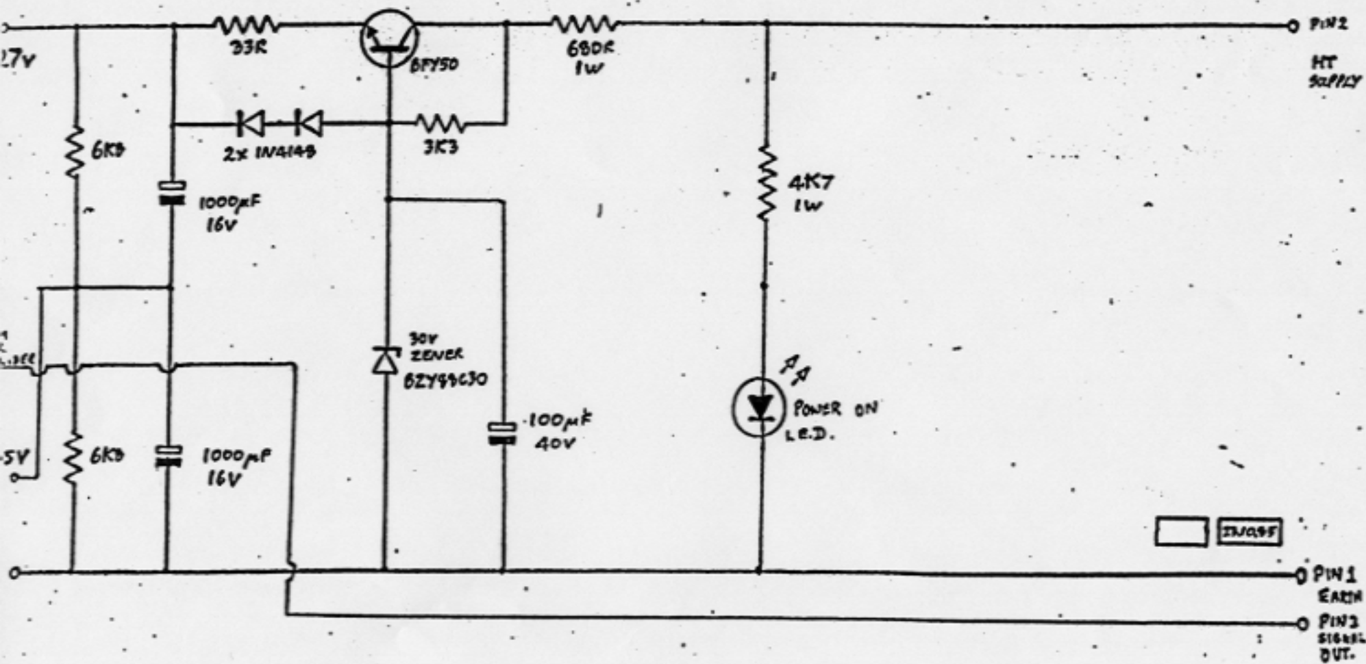
② TRACE ELLIOT G.P 7 POWER SUPPLY.
