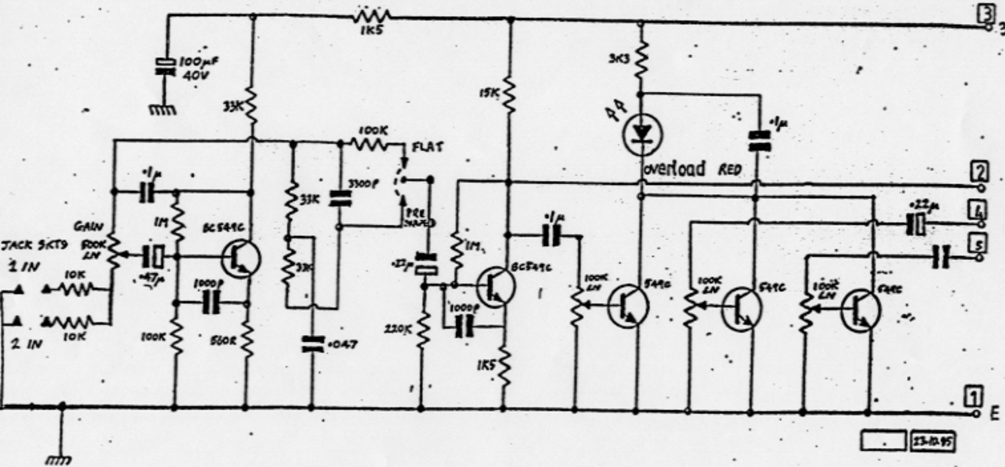
(10) TRACE ELLIOT GP 7 INPUT MATCHING STAGE
